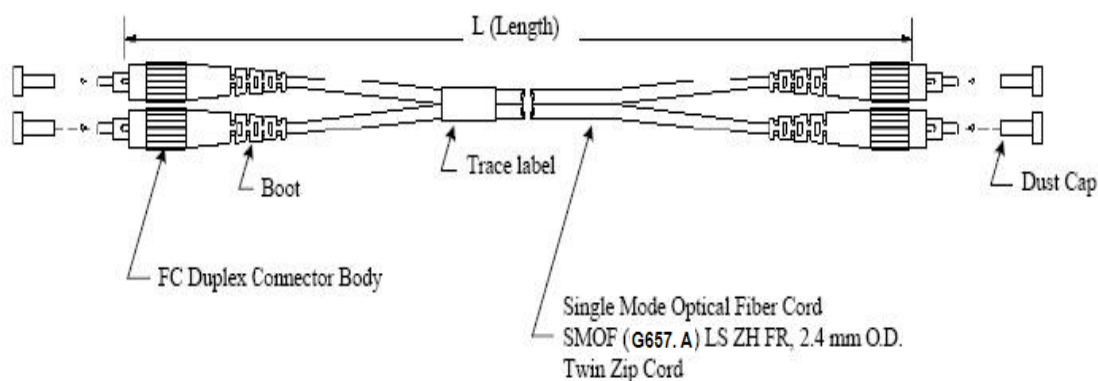
Figure 9 FC to FC Single Mode Fiber Patch Cord Duplex
