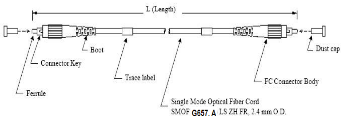
Figure 3 FC to FC Single Mode Fiber Patch Cord
