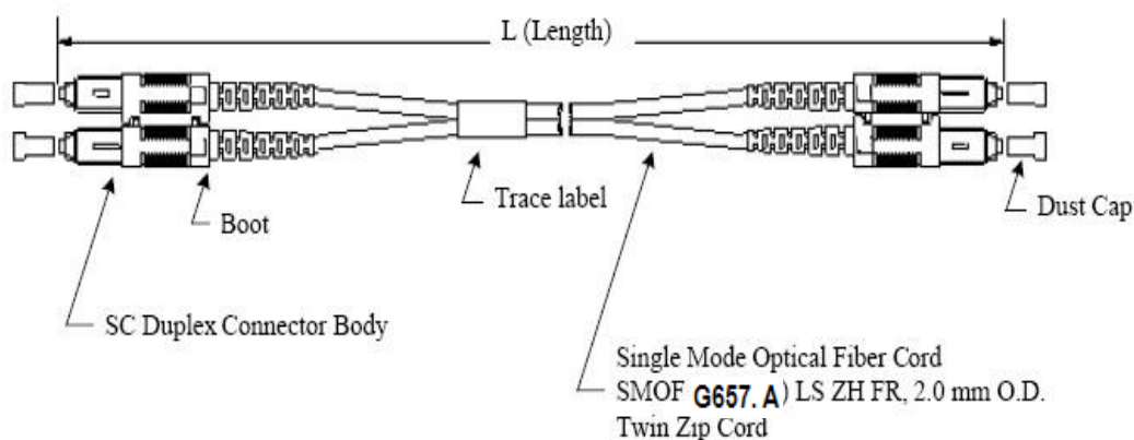
Figure 10 SC to SC Single Mode Fiber Patch Cord Duplex
