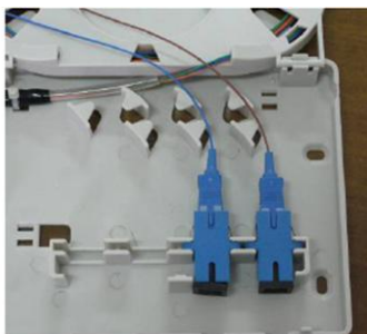
Pic11: install the adaptor and pigtail Pic12: put the pigtail through into the inlet port Pic13: pigtail inserted the tray
