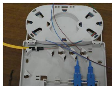
Pic11: install the adaptor and pigtail Pic12: put the pigtail through into the inlet port Pic13: pigtail inserted the tray
