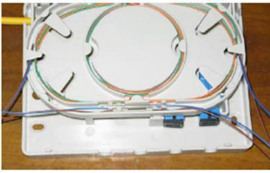
Pic14: after shrink, splice protective tube put into the slot
