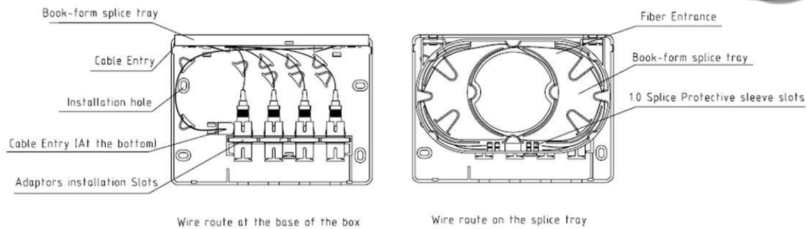
Pic1: The fiber route schematic diagram
