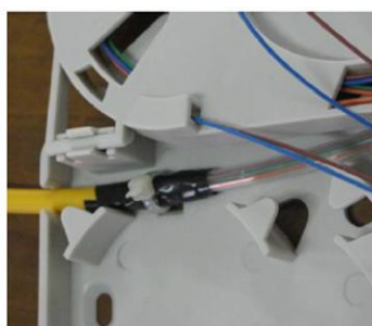
Pic11: install the adaptor and pigtail Pic12: put the pigtail through into the inlet port Pic13: pigtail inserted the tray
